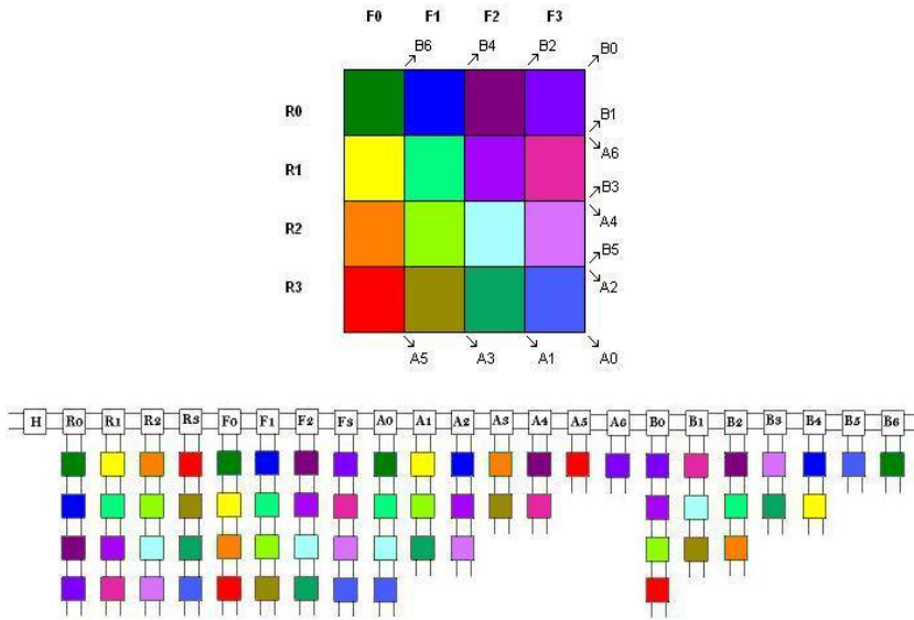
Figure 3: Chessboard and Corresponding Universe
